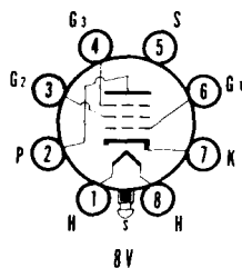
SYLVANIA TYPE 7B7 REMOTE CUTOFF PENTODE
