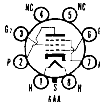
SYLVANIA TYPE 35A5 BEAM POWER AMPLIFIER
