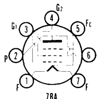
SYLVANIA TYPE 3Q4 BEAM POWER AMPLIFIER
