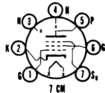
SYLVANIA TYPE 6BZ6 SEMI-REMOTE CUTOFF PENTODE
