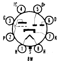
SYLVANIA TYPE 7B6 DUODIODE HIGH-MU TRIODE
