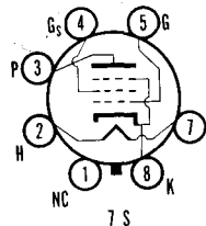
SYLVANIA TYPE 50L6GT BEAM POWER AMPLIFIER
